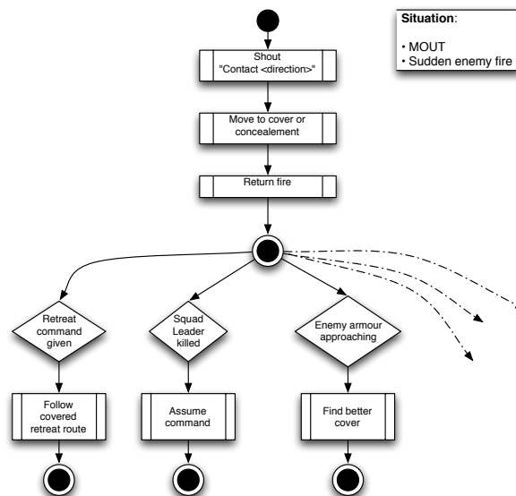
Figure 1. Graphical plan in CoJACK.
